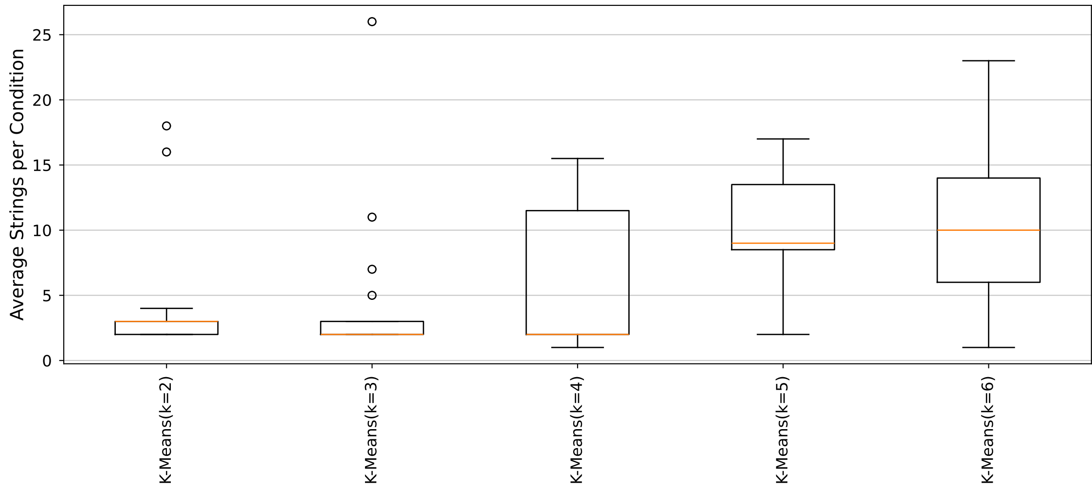
YARA Rules Average Strings per Condition Distribution (Cluster22_Size6 dataset)
